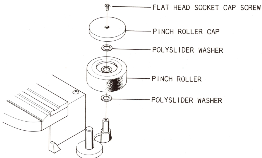
Figure 8-4 Pinch Roller Removal
