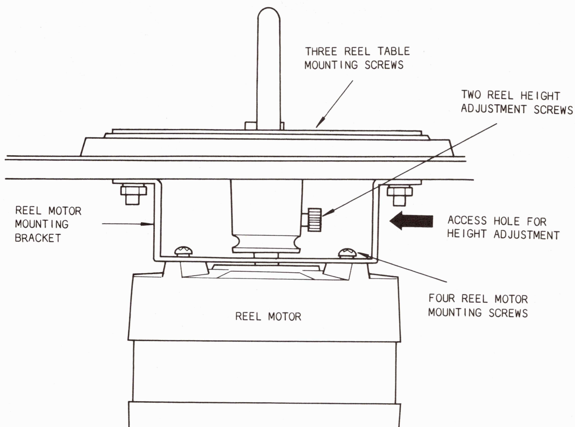
Figure 8-1 Reel Motor Mounting
