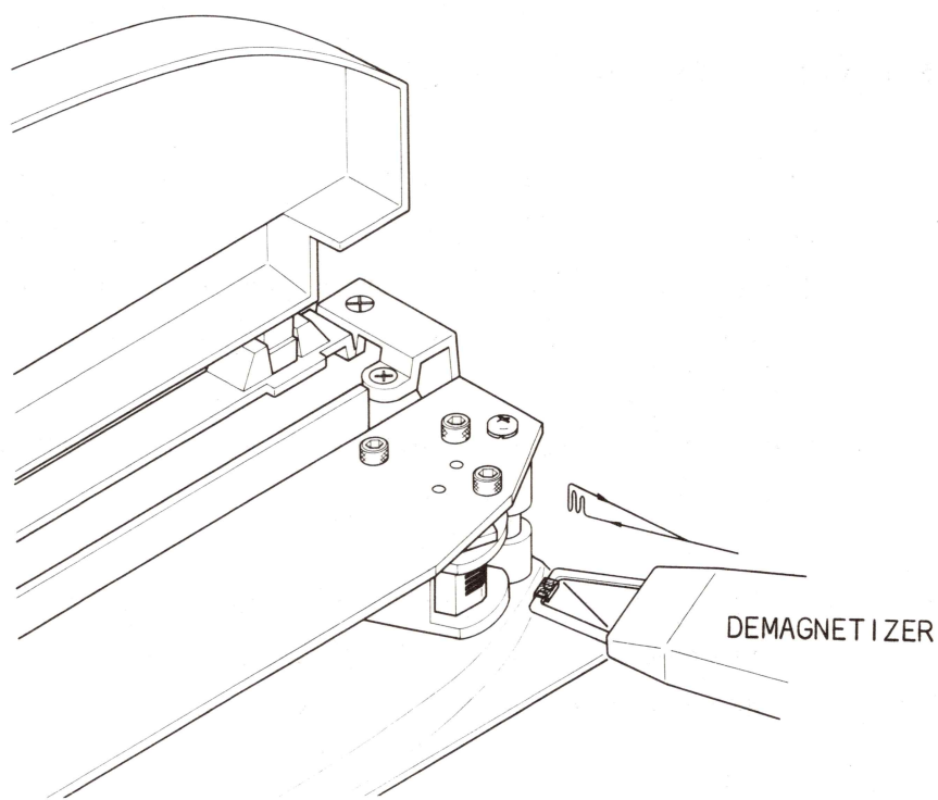
Figure 5-2 Demagnetizing
