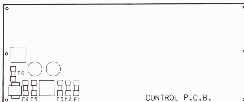
Figure 5-6 Internal Fuse Location
