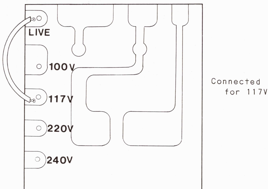
Figure 5-4 Voltage Selection Terminal
