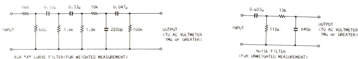
Figure 7-1 Filter Schematics
