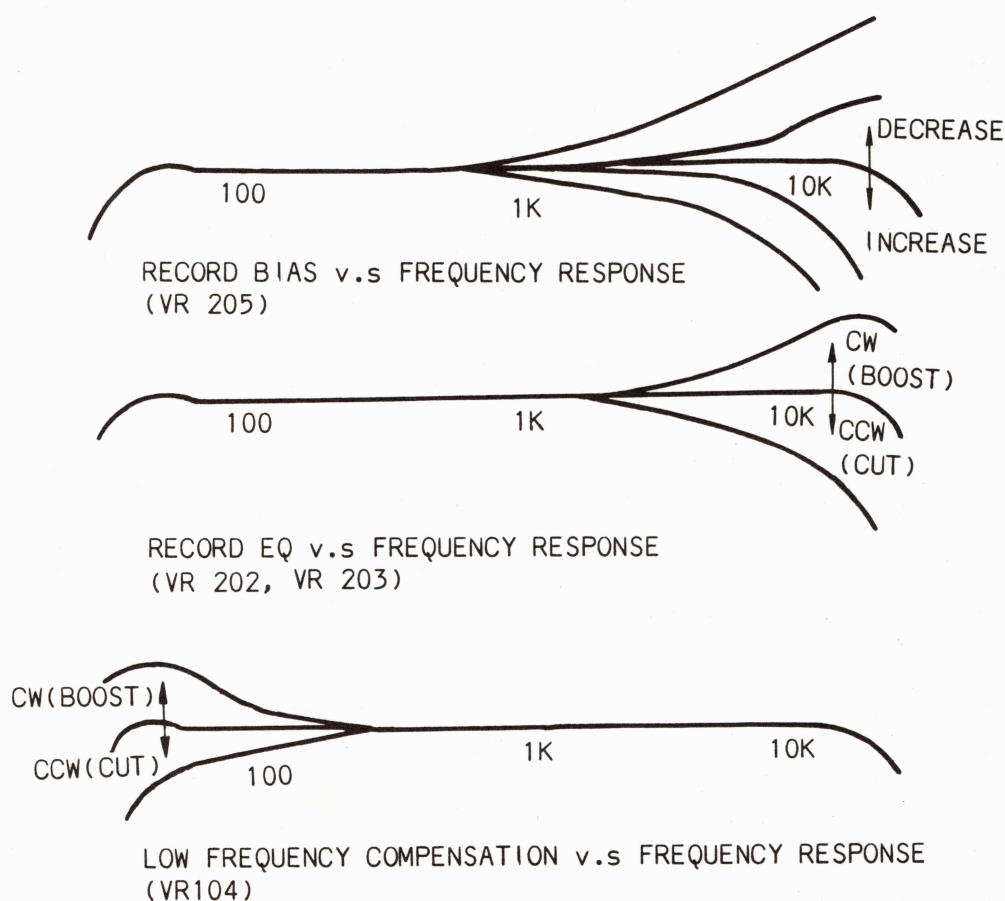
Figure 7-7 Overall Frequency Response
