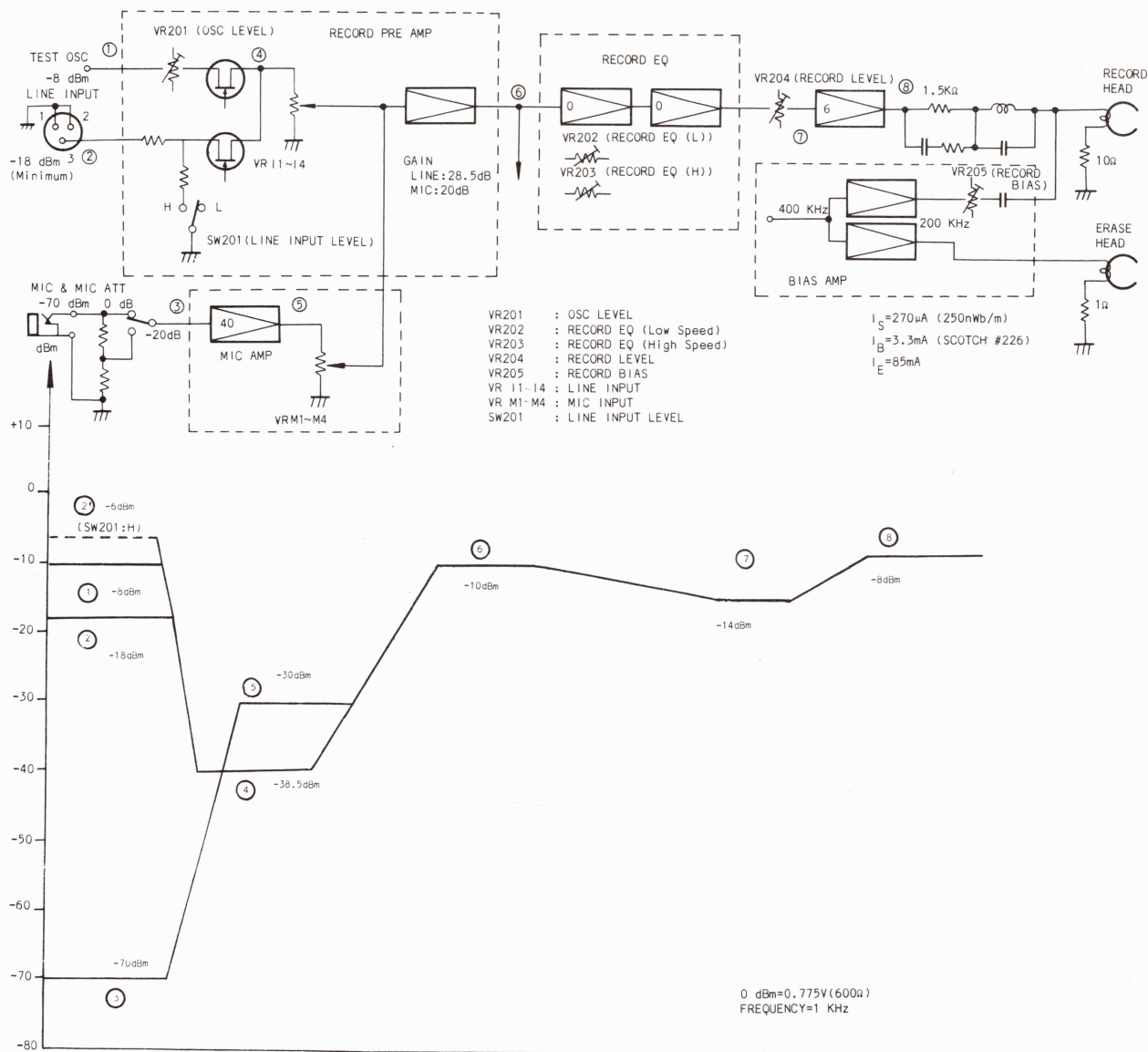
Figure 7-8 Record System Block and Level Diagram
