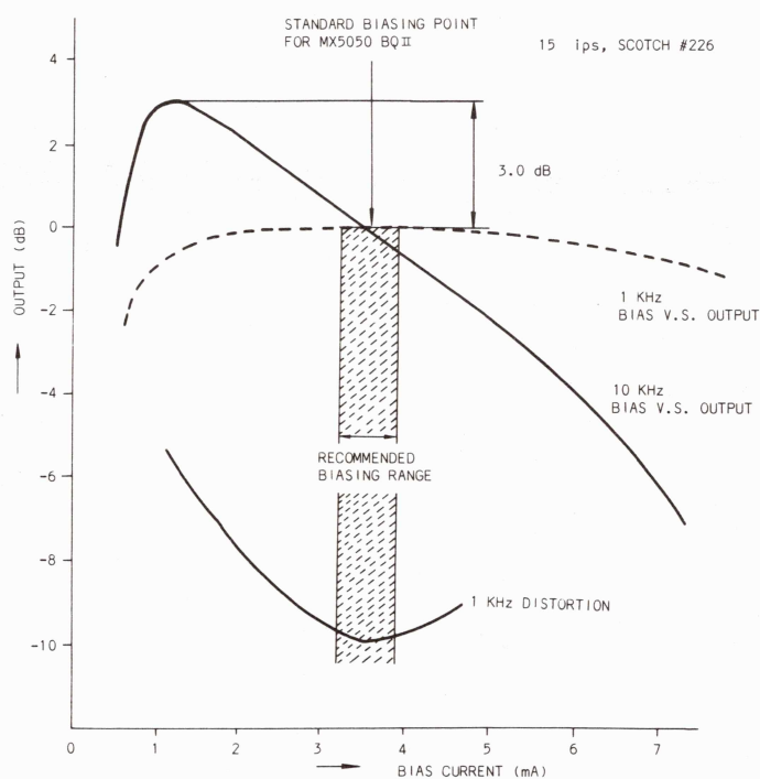
Figure 7-9 Bias Current v.s. Output and Distortion
