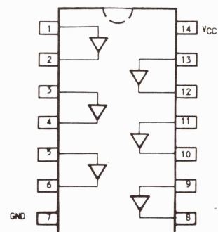
IC-25 1A07N (SN7407N)
