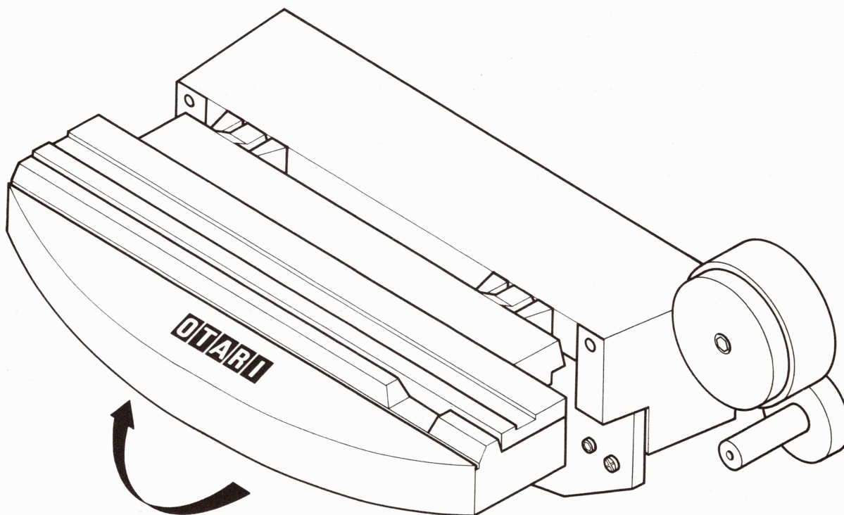
Figure 5-1 Lifting the Head Cover
