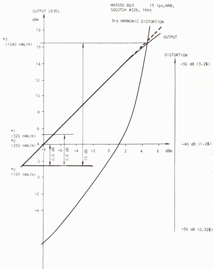
Figure 7-10 Input v.s. Output and Distortion
