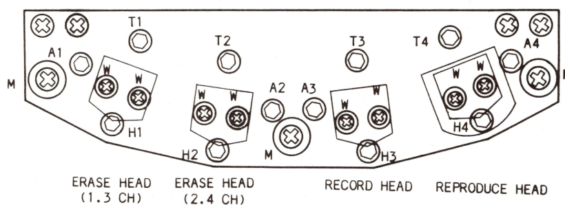
Figure 8-5 Head Assembly
