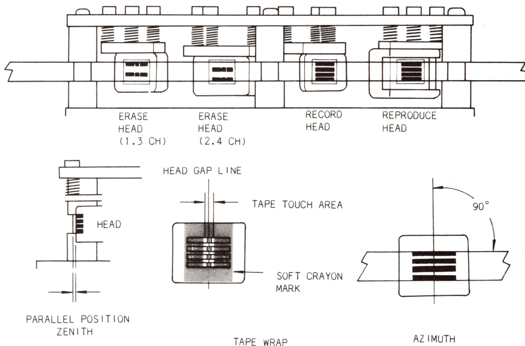
Figure 8-6 Head Alignment
