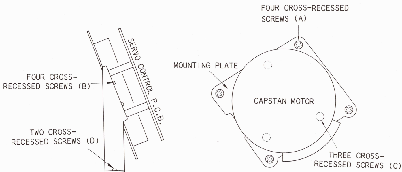
Figure 8-3 Location of DC Servo Capstan Motor
