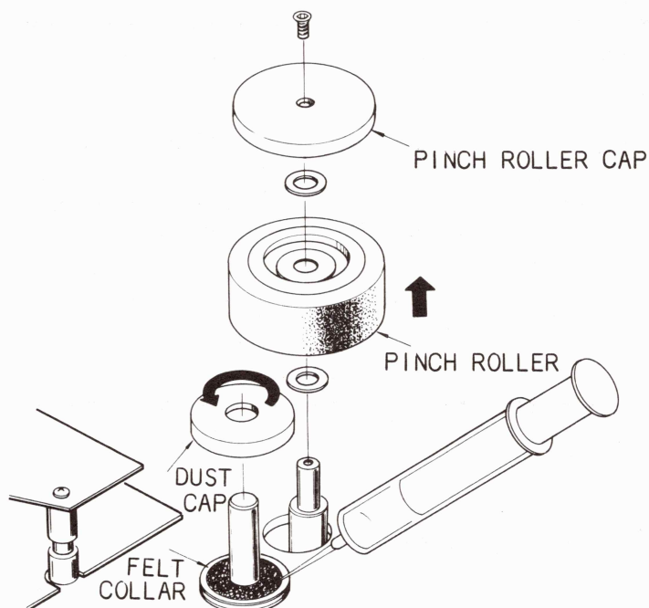
Figure 5-3 Lubrication
