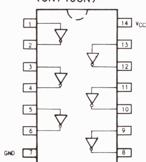
IC-24 1ALS05N (SN74LS05N) 1A06N (SN7406N)
