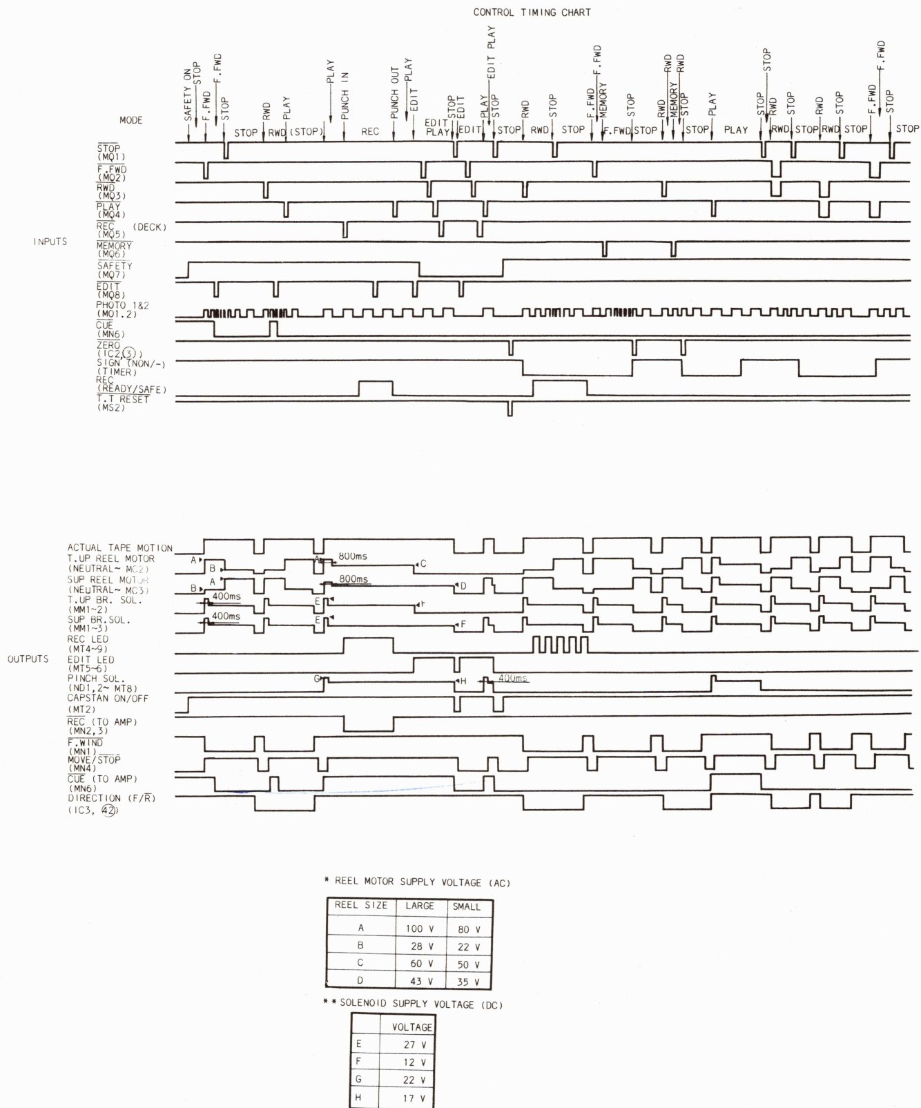
Figure 6-7 Control Timing Chart
