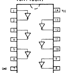
IC-24 1ALS05N (SN74LS05N) 1A06N (SN7406N)
