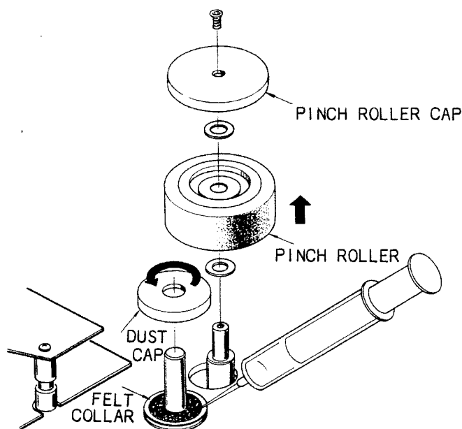
Figure 5-3 Lubrication
