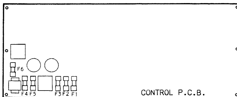
Figure 5-6 Internal Fuse Location
