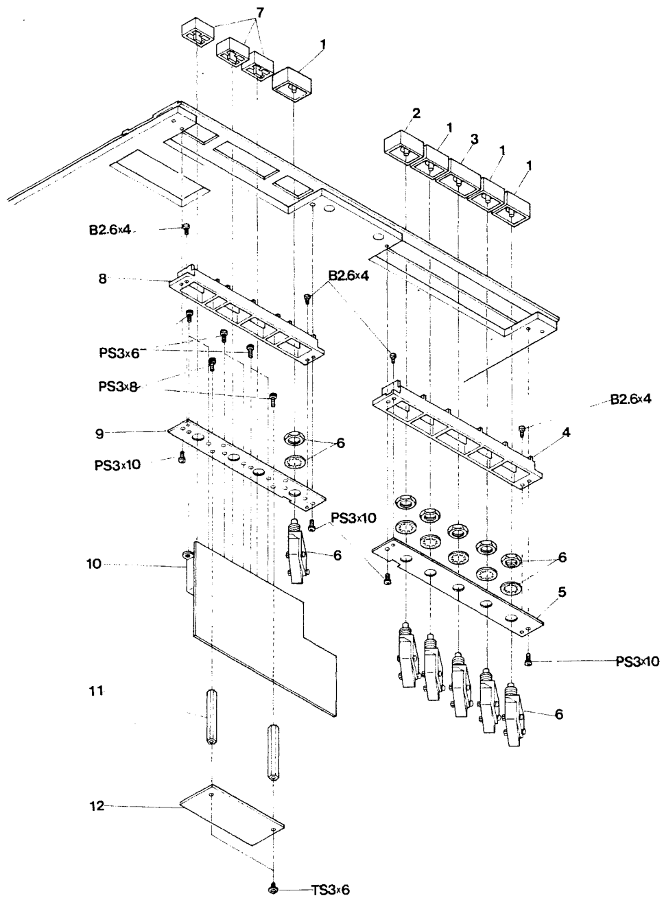
EXPLODED VIEW 6. CONTROL SWITCH ASSEMBLY
