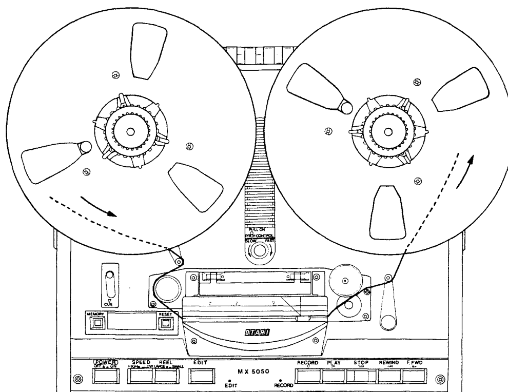
Figure 3-2 Tape Threading
