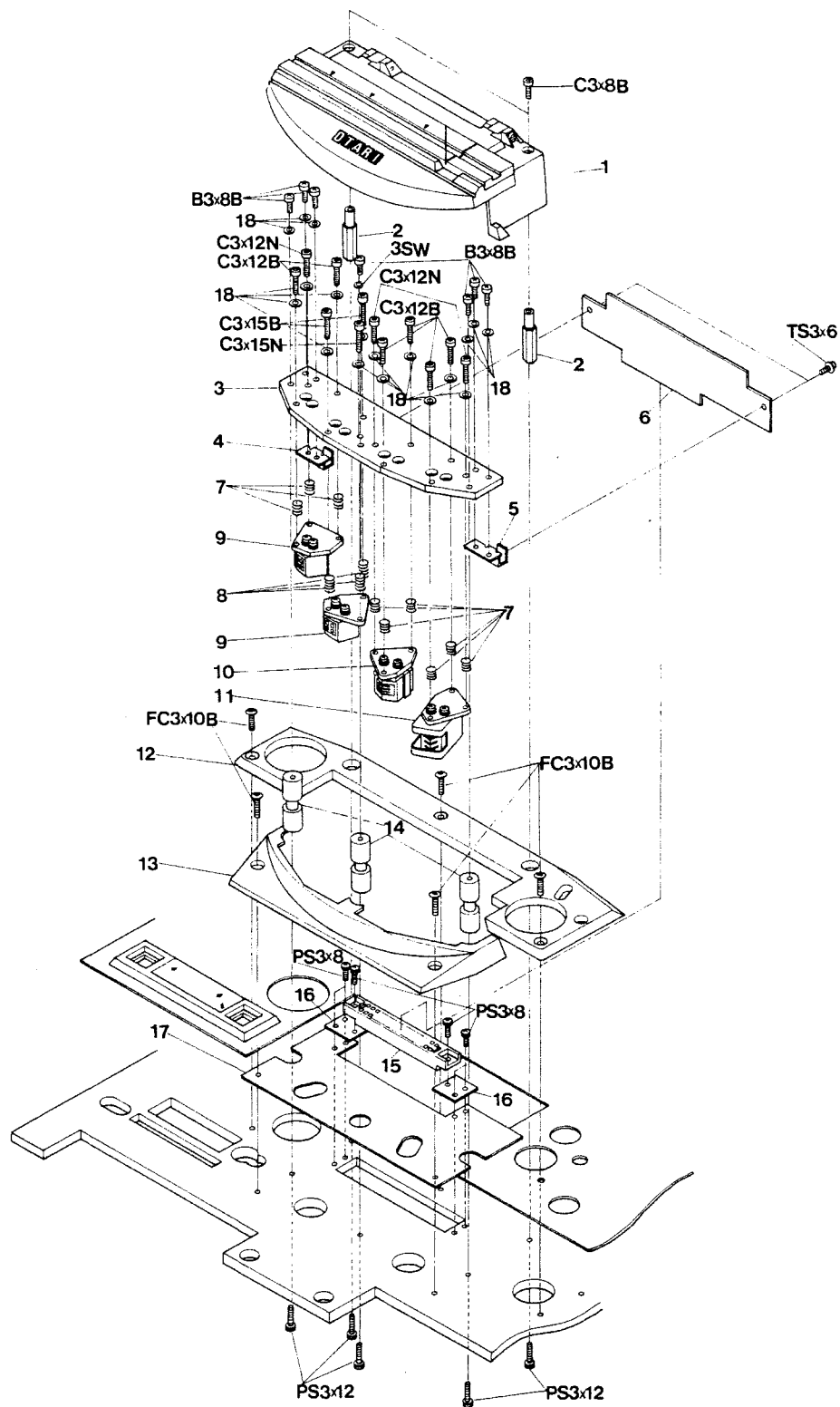
EXPLODED VIEW 1. HEAD ASSEMBLY
