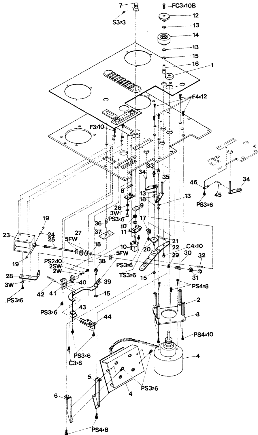
EXPLODED VIEW 3. CAPSTAN, PINCH ROLLER and SHIFTER ASSEMBLY
