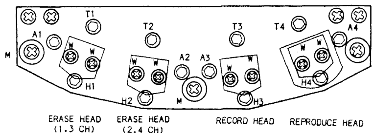
Figure 7-5 Head Assembly
