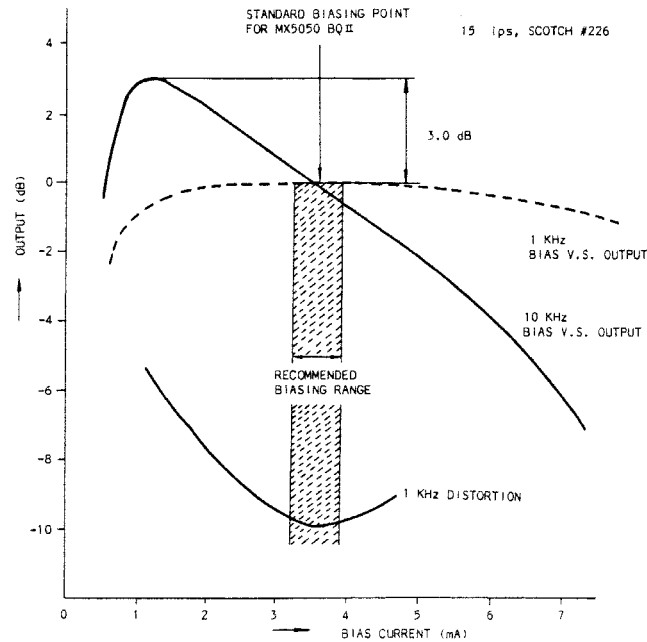
Figure 7-9 Bias Current vs. Output and Distortion
