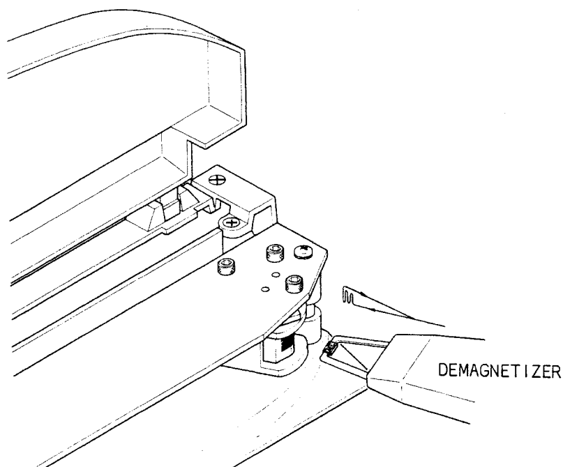
Figure 5-2 Demagnetizing
