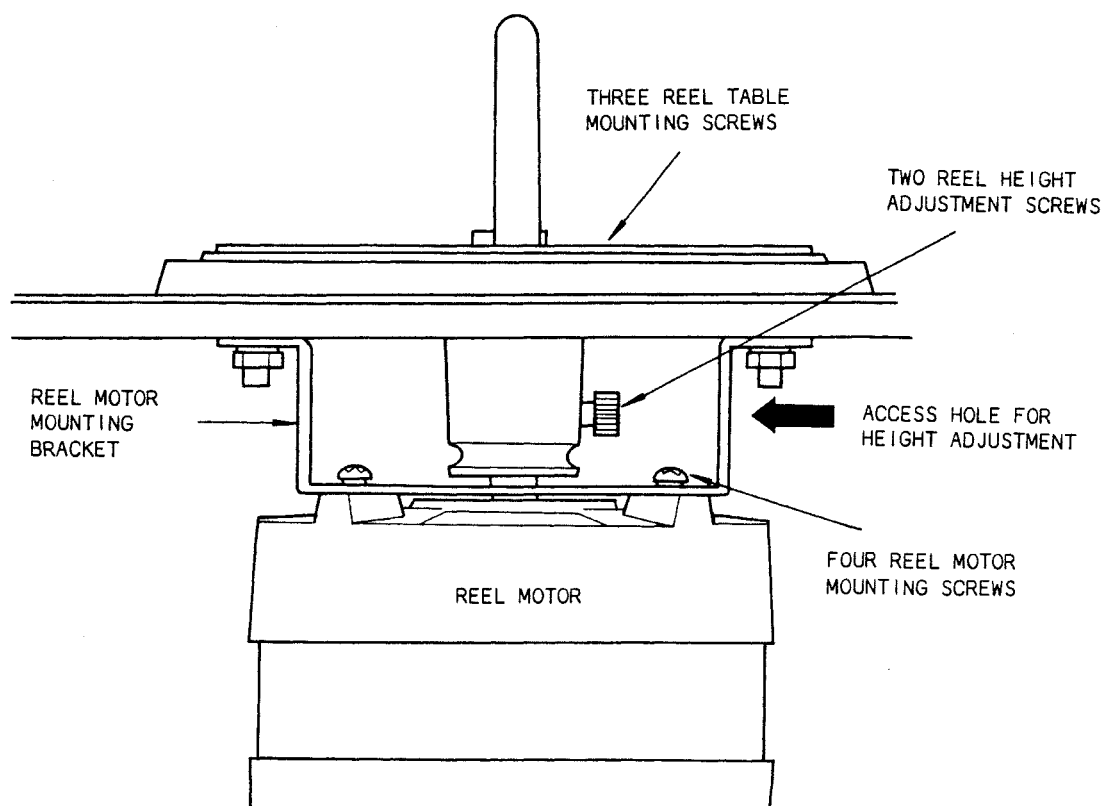
Figure 8-1 Reel Motor Mounting
