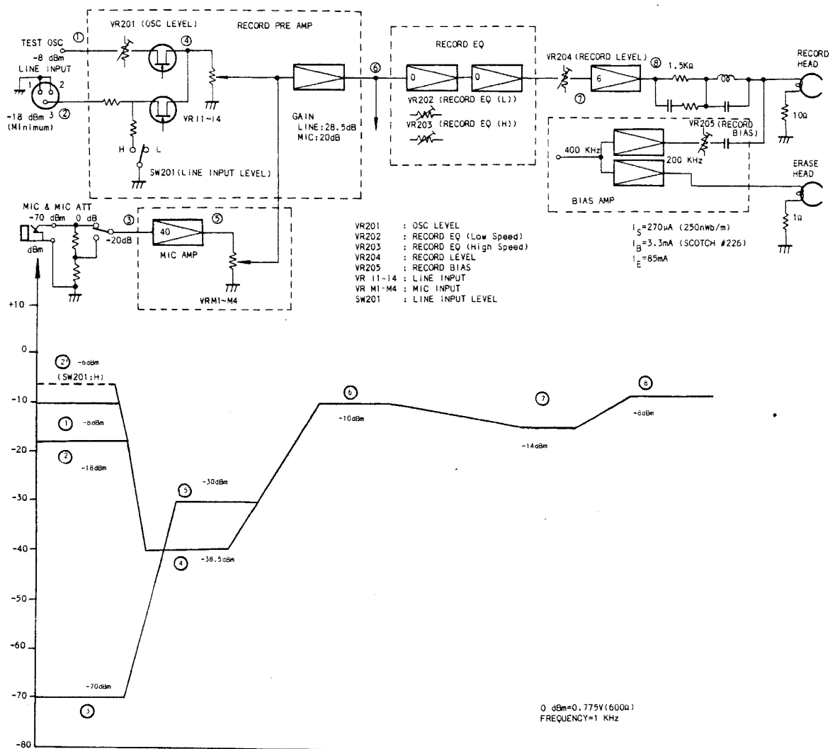
Figure 7-8 Record System Block and Level Diagram
