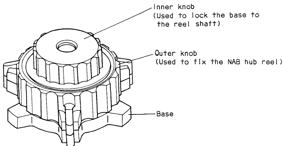
Figure 3-1 Reel Hold Down Knob
