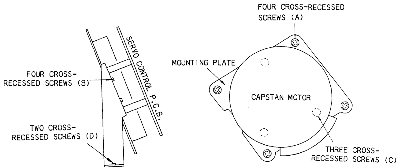
Figure 8-3 Location of DC Servo Capstan Motor
