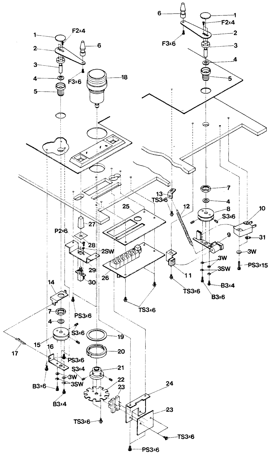
EXPLODED VIEW 5. TENSION ARM, IMPEDANCE ROLLER, and TIMER ASSEMBLY
