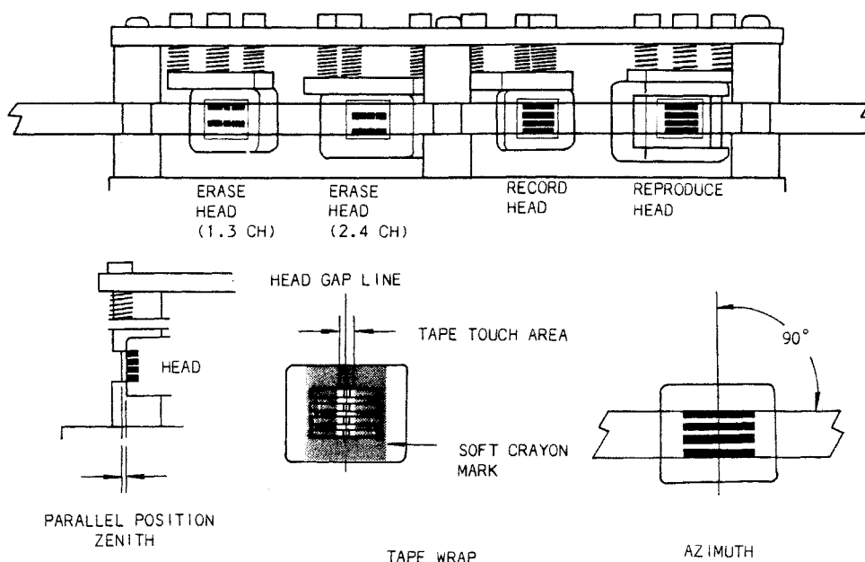
Figure 8-6 Head Alignment
