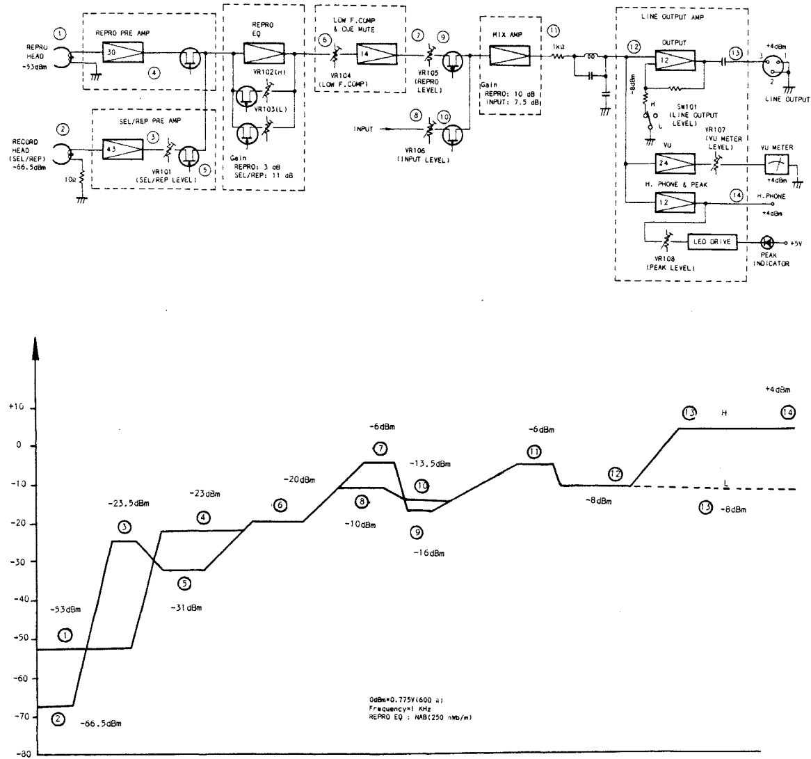
Figure 7-4 Reproduce System Block and Level Diagram
