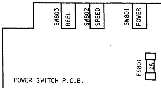
Figure 5-5 Main Power Fuse Location
