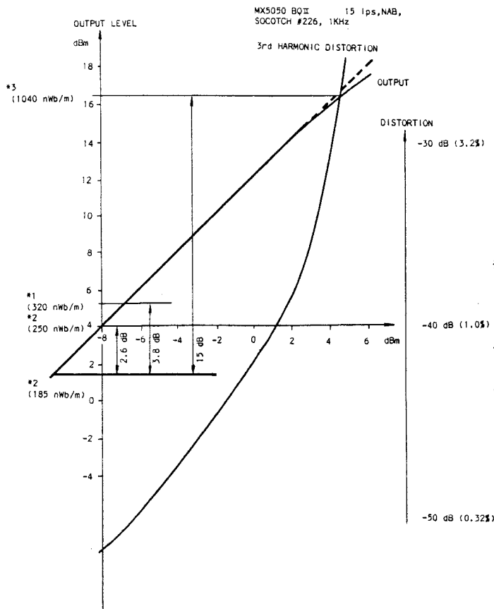
Figure 7-10 Input vs. Output and Distortion
