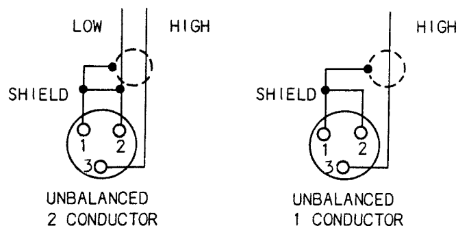
Figure 2-5 Input/Output Assembly Connector Wiring
