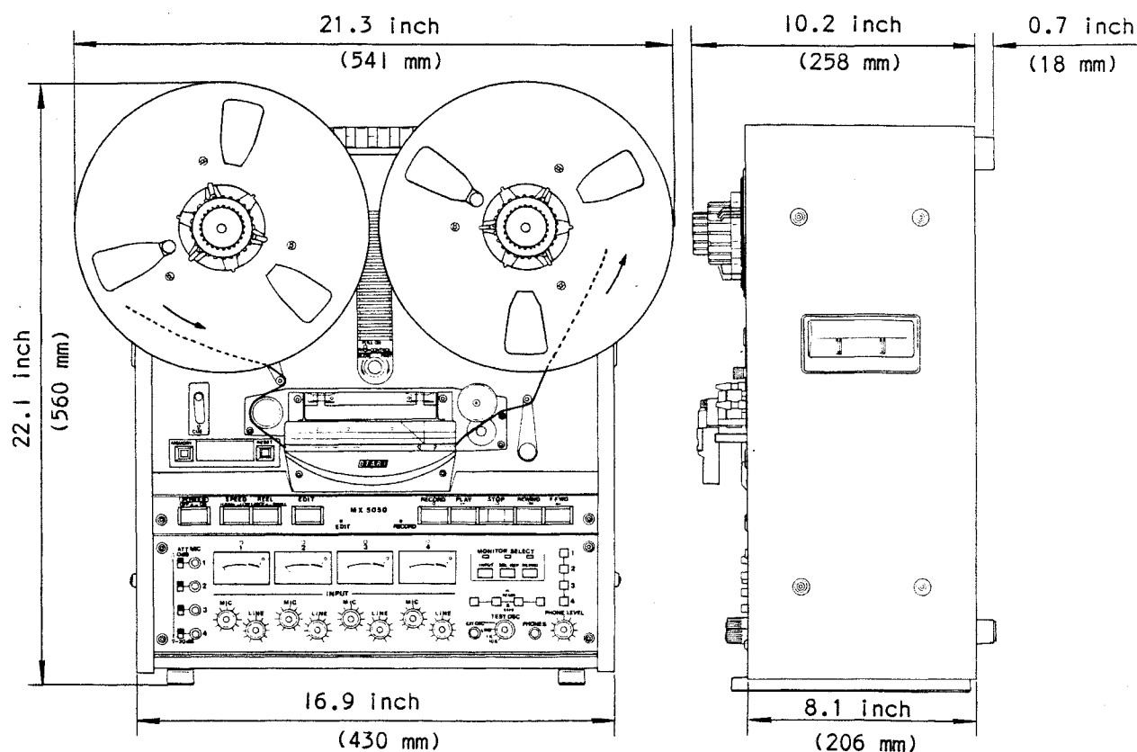
Figure 2-1 Dimensions
