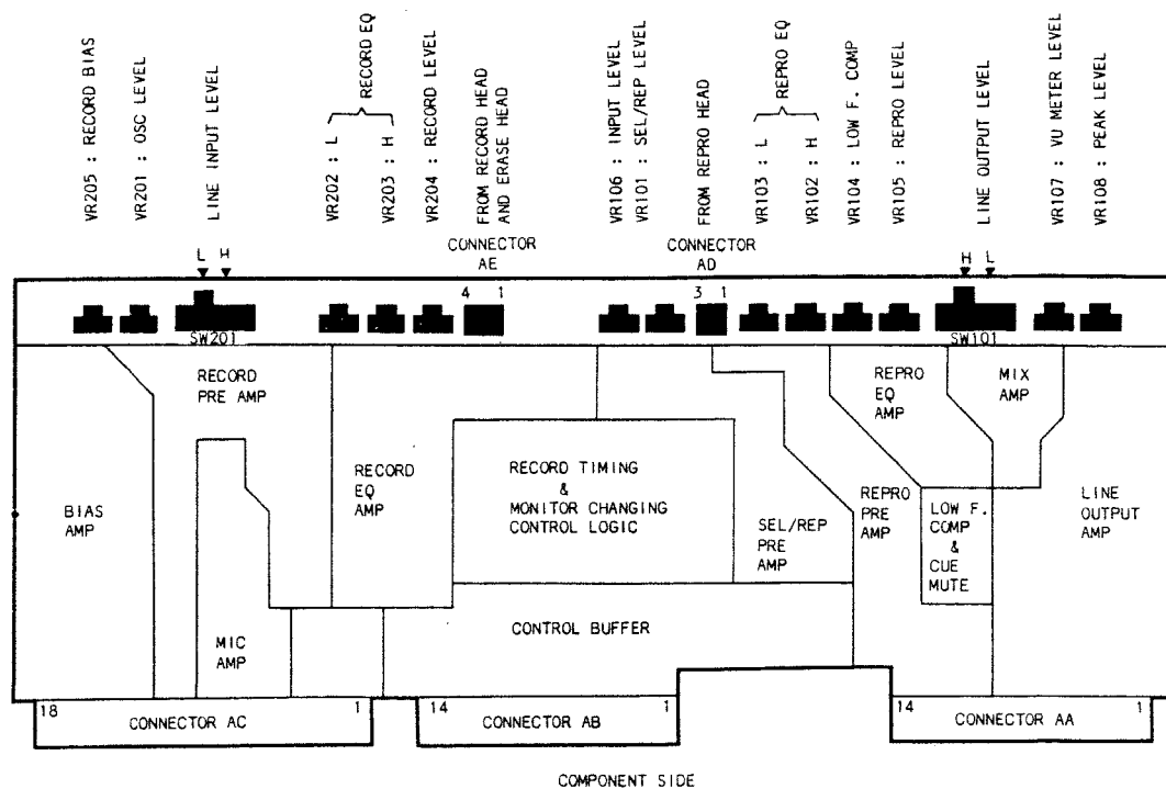
Figure 7-1' Location of Record/Reproduce Electronics
